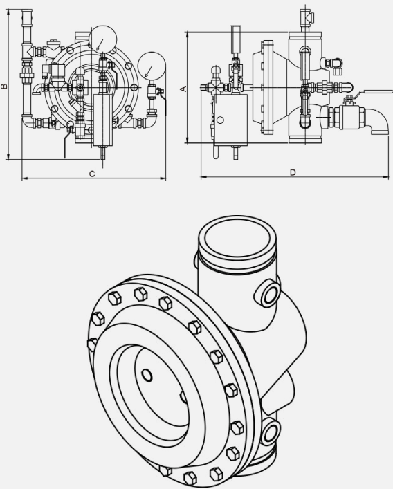
Figure 3 Outline dimensional drawing of deluge valve (Grooved connection)
