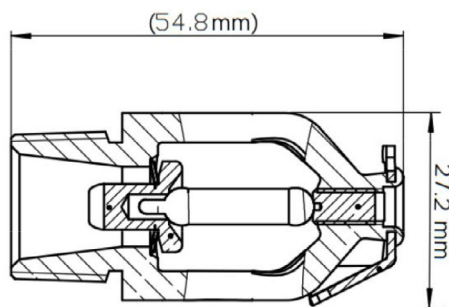
Sidewall Sprinkler Dimension
