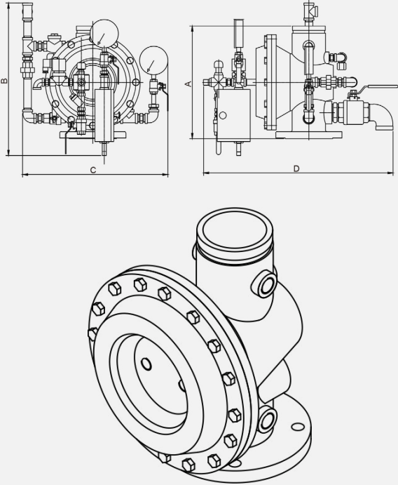
Figure 2 Outline dimensional drawing of deluge valve (Grooved * Flange connection)
