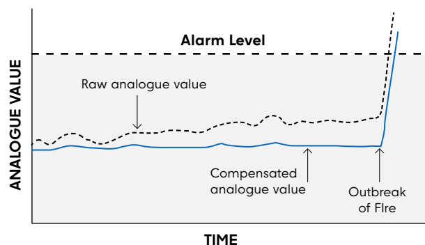
Figure 1 – Drift Compensation Graph
